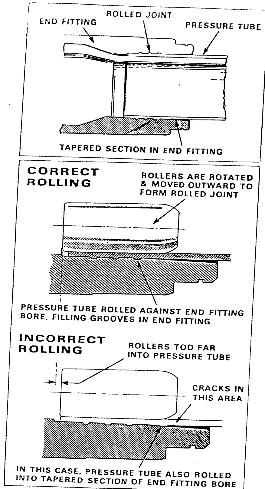
FIGURE 9 SCHEMATIC DRAWING TO ILLUSTRATE CORRECT AND INCORRECT ROLLING OF PRESSURE TUBE INTO THE END FITTING
