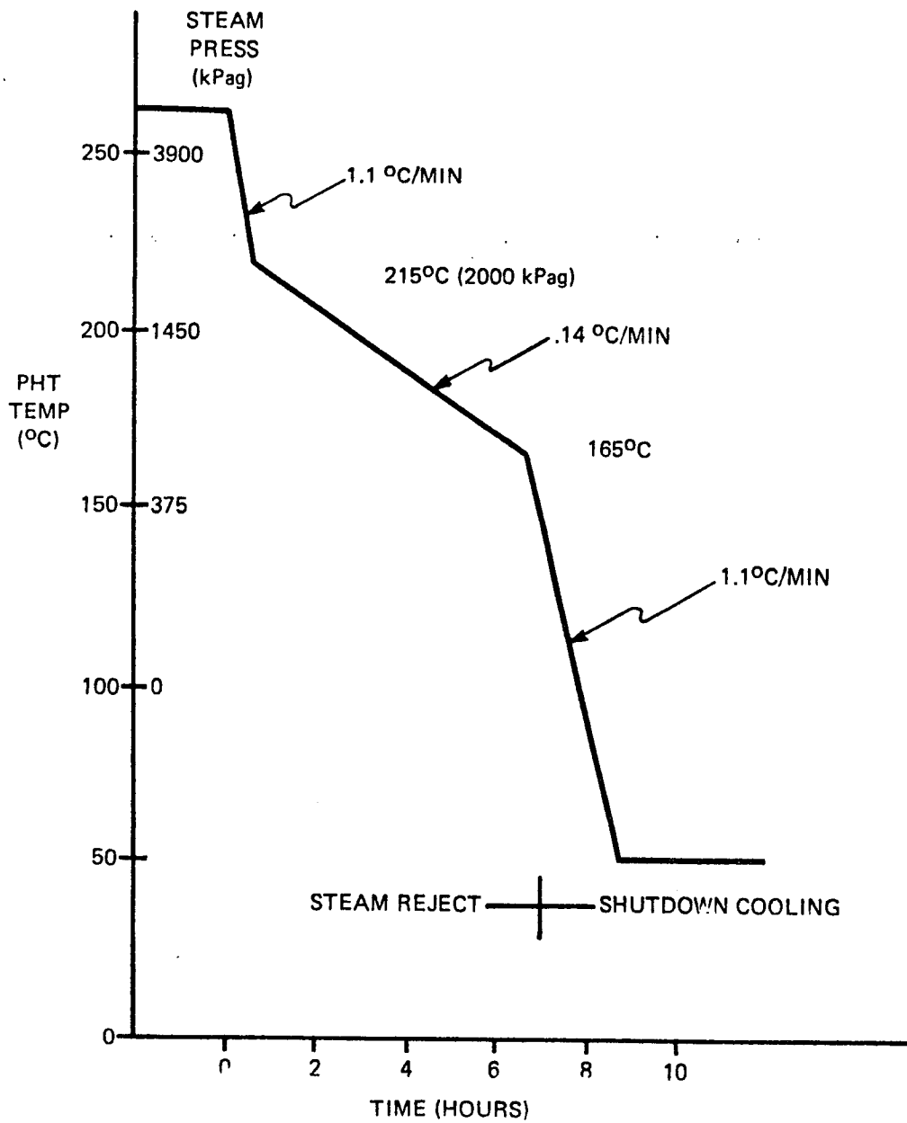
FIGURE 4: COOLDOWN TEMPERATURE PROFILE
