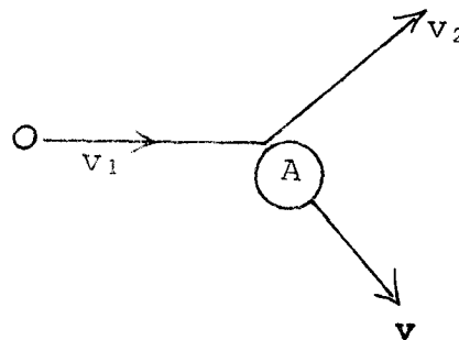
Figure 1 Elastic Collision
