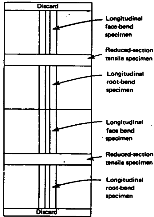
QW-463.1(b) PLATES — 1/4 IN. AND OVER THICKNESS AND ALTERNATE FROM 1/8 IN. BUT LESS THAN 1/4 IN. THICKNESS PROCEDURE QUALIFICATION
