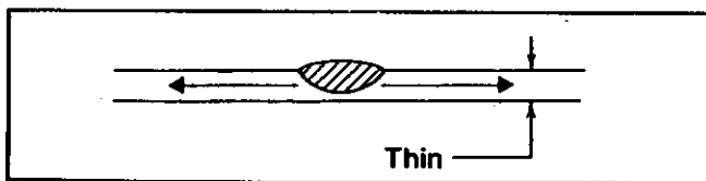
Fig. 9 — Thin plate showing a slower cooling rate. The heat is transferred in two directions.
