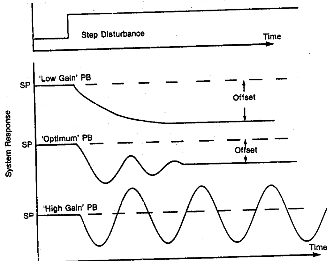
Figure 3: Responses to Varying Proportional Gains.
