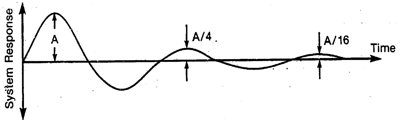
Figure 1: Typical 1/4 Decay Response.
