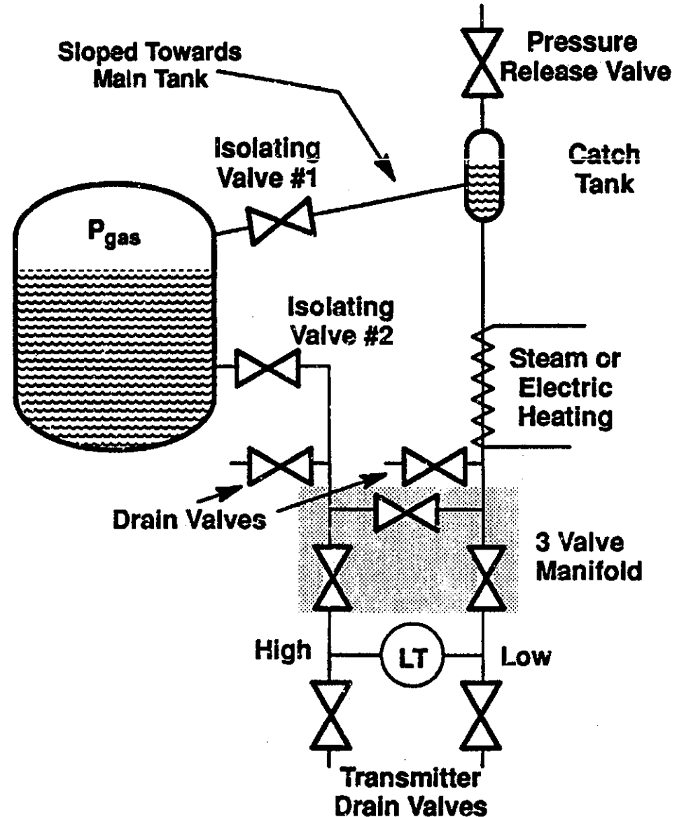
Figure 5: A Wet Leg Installation.
