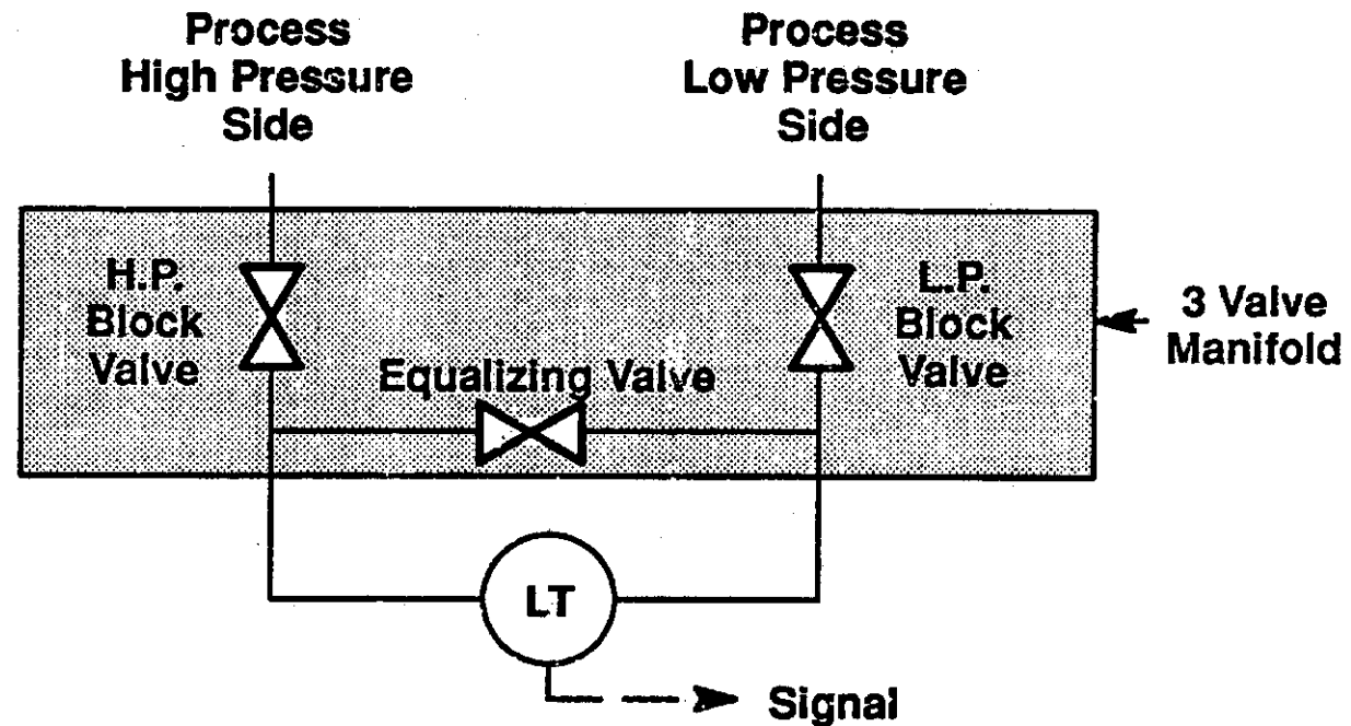
Figure 3: A Three Valve Manifold.
