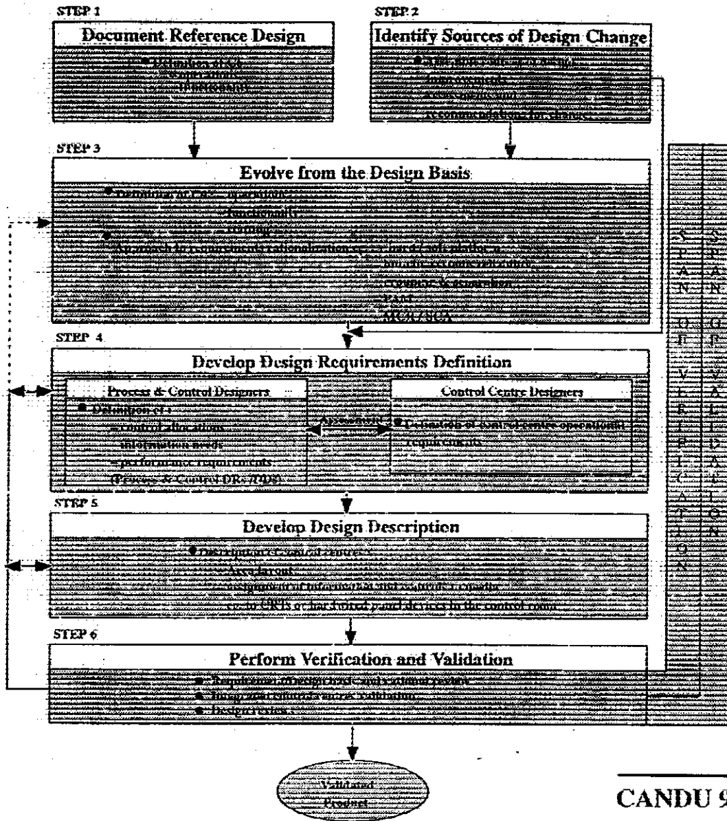
The CANDU 9 HFE Level A Design Process Logic FlowChart
