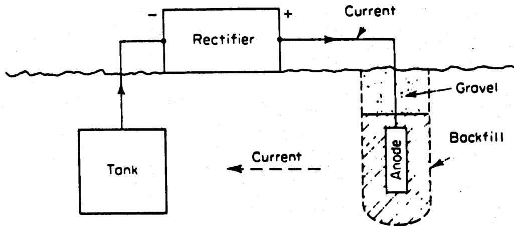
Cathodic protection of an underground tank using impressed currents.
