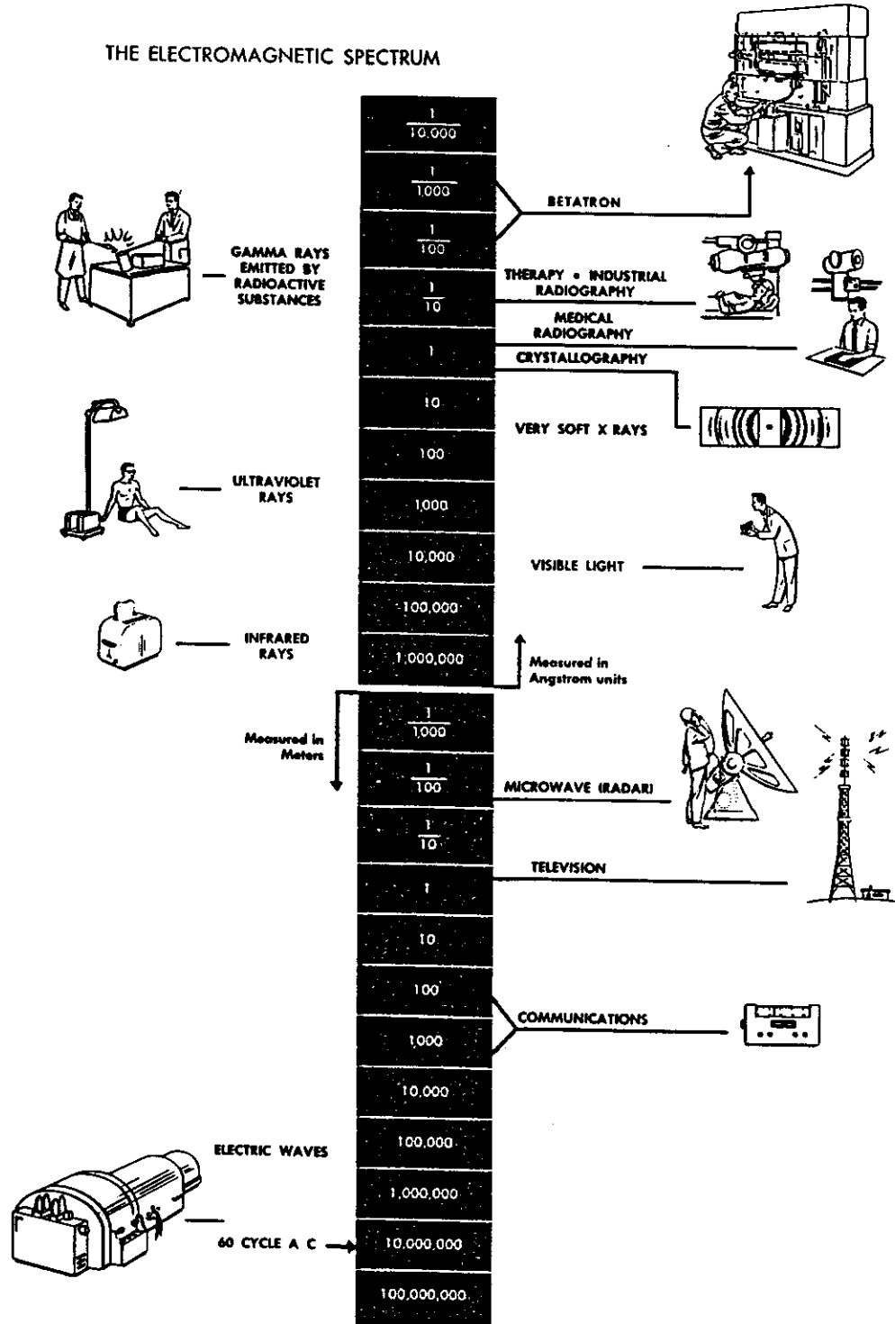
Figure 1.1: The Electromagnetic Spectrum
