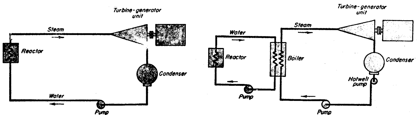
Direct Cycle
