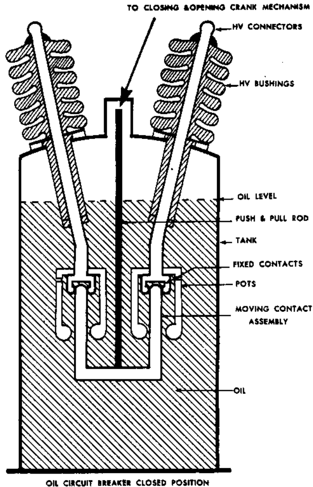
Figure 1: Diagram Showing a Section of an HV Oil Circuit Breaker in the Closed Position.
