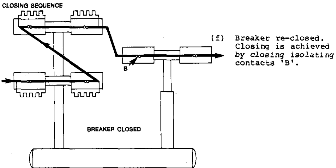
Figure 5 (Continued): Air Blast Circuit Breaker Operating Sequences.
