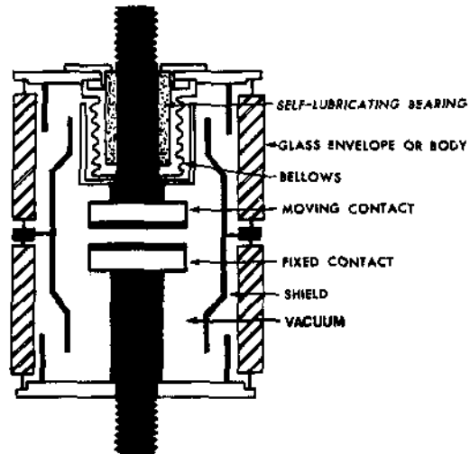
VACUUM CONTACTOR OPEN POSITION
