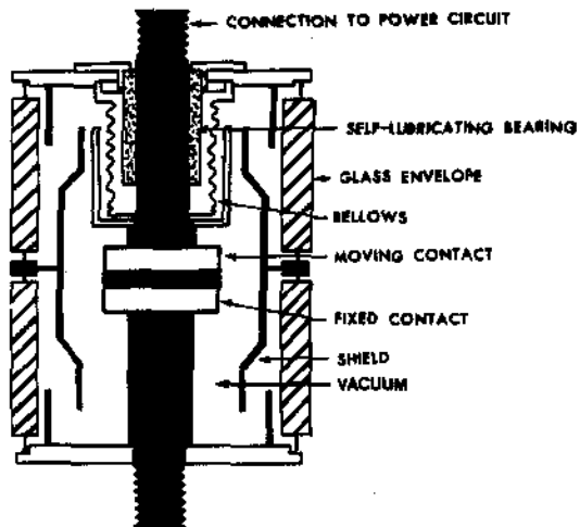
VACUUM CONTACTOR CLOSED POSITION
