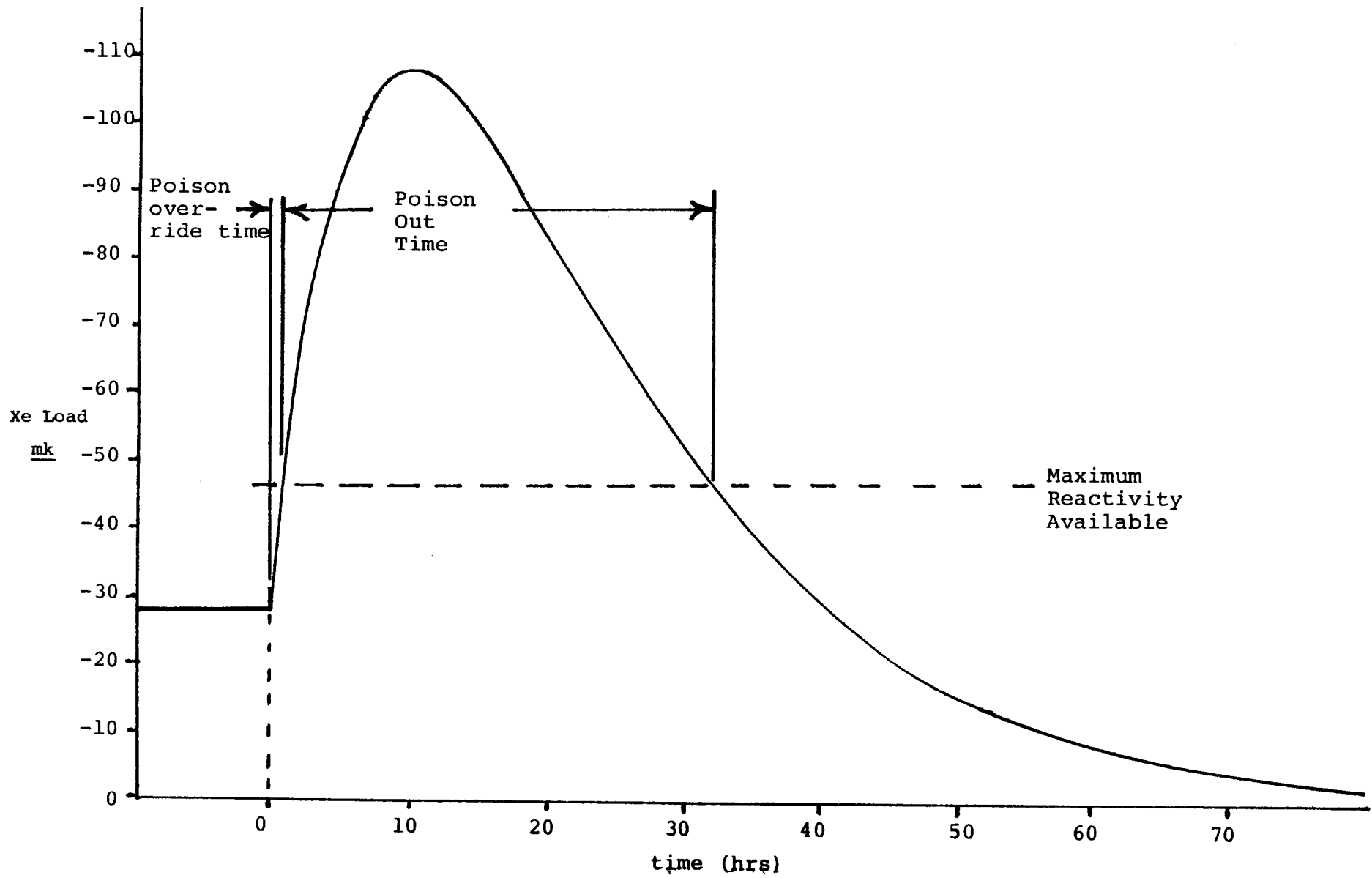
Behaviour of Xenon Load after a trip from full power.
