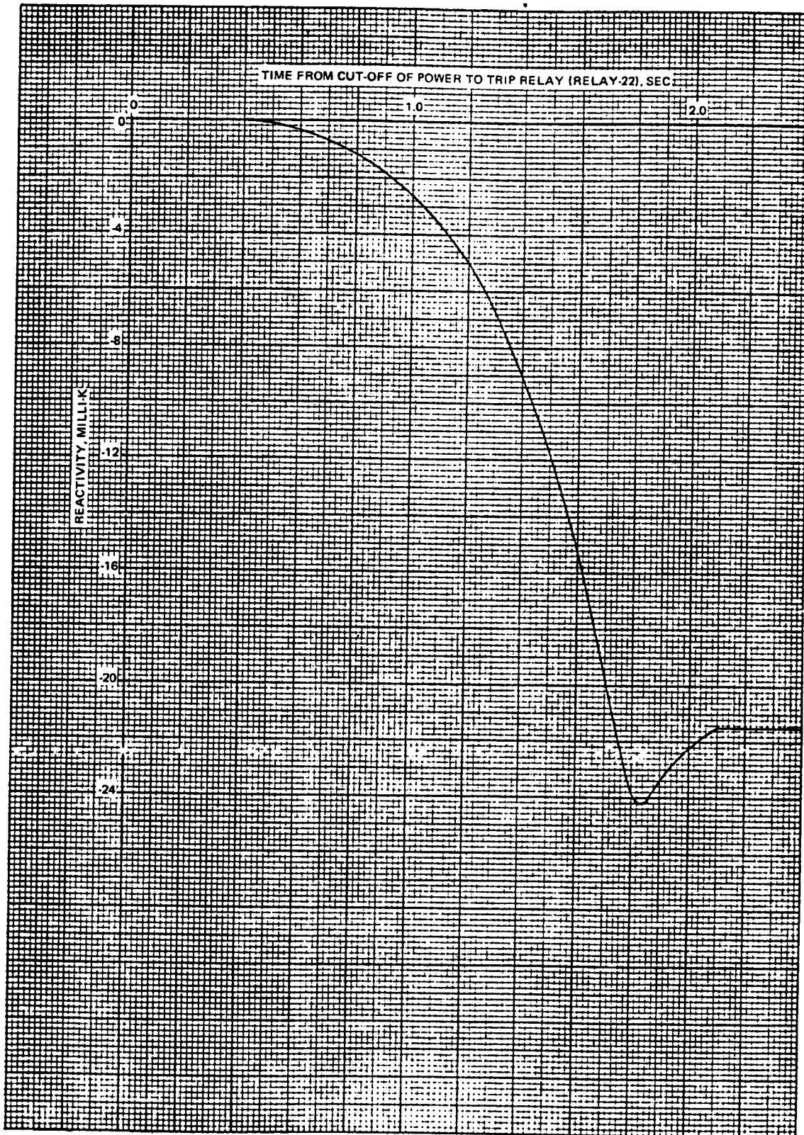
REACTIVITY VERSUS TIME FROM TRIP SIGNAL (RELAY-22) FOR SHUT-OFF ROD DROP AT FULL MODERATOR LEVEL, EQUILIBRIUM FUEL CONDITIONS
