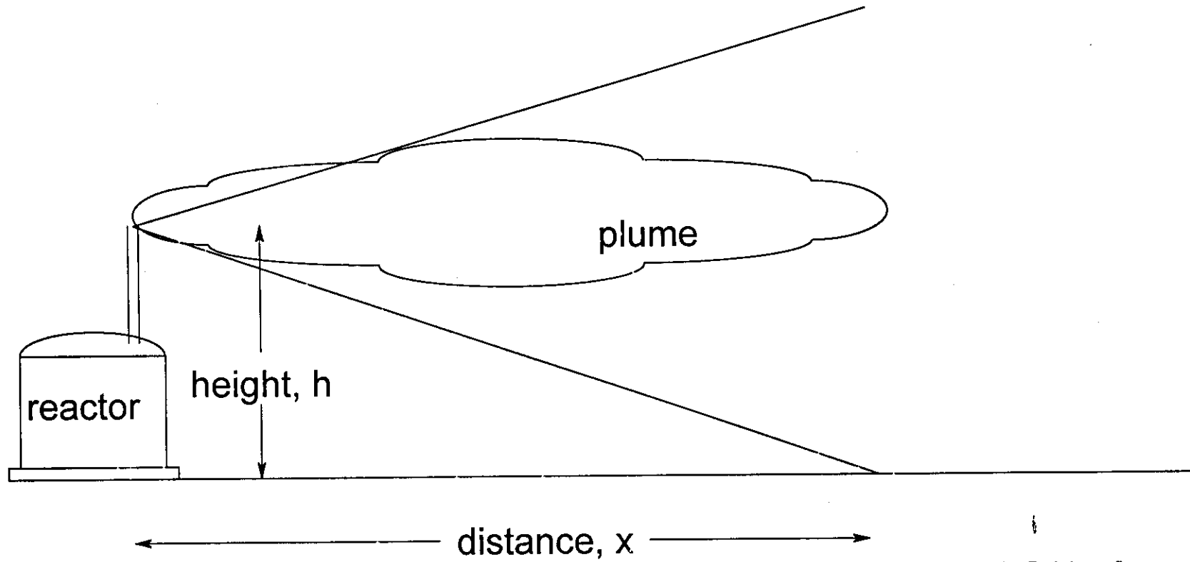
Figure 6.2 Dispersion of effluents
