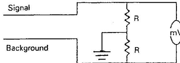
Fig. 1. Schematic of SPND with automatic background subtraction.
