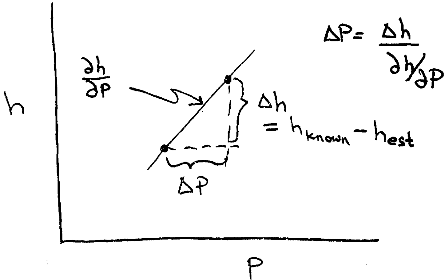
Figure 4.3 Error correction scheme for pressure in two-phase.
