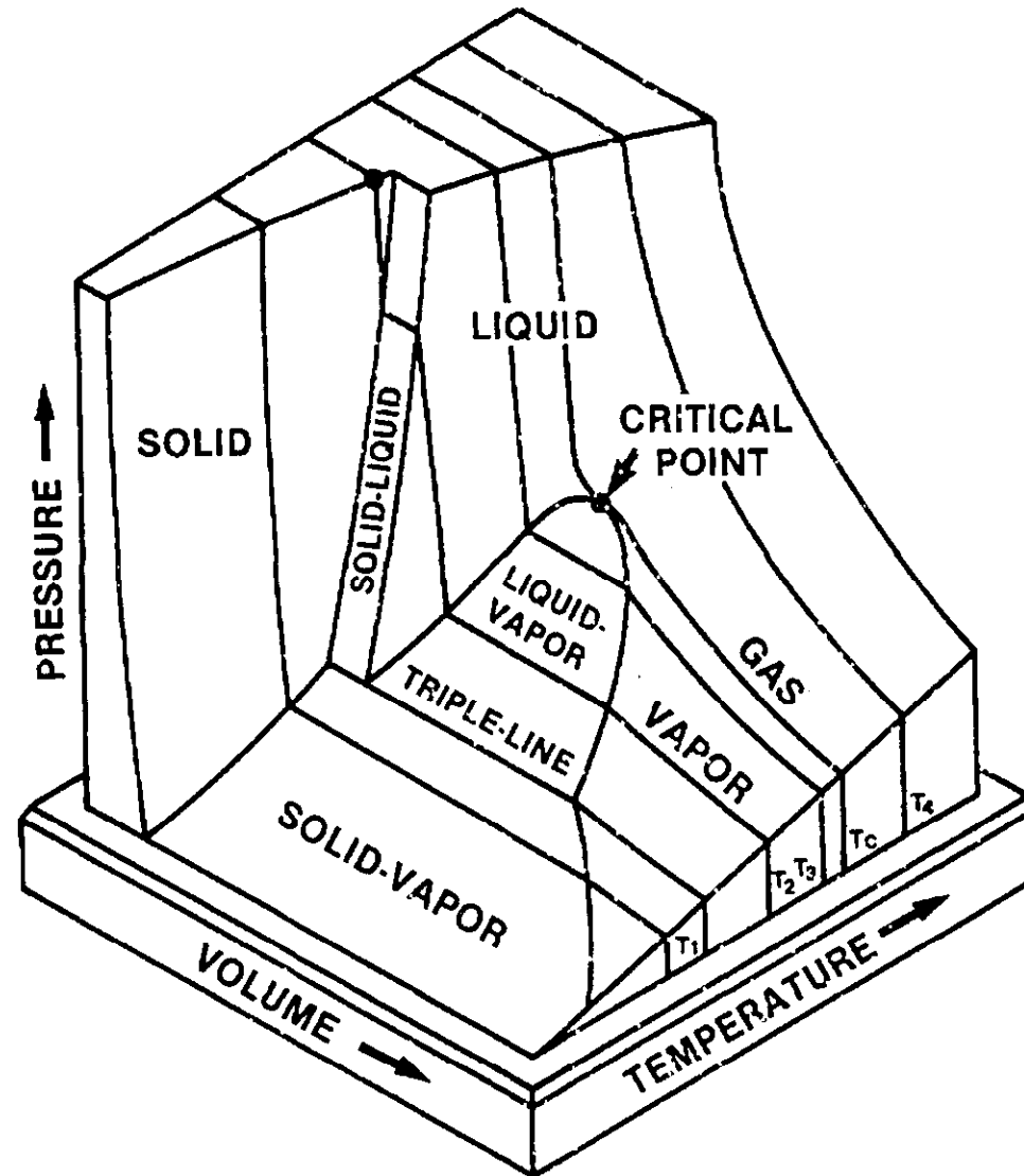
Figure 4.1 P-v-T surface for water.
