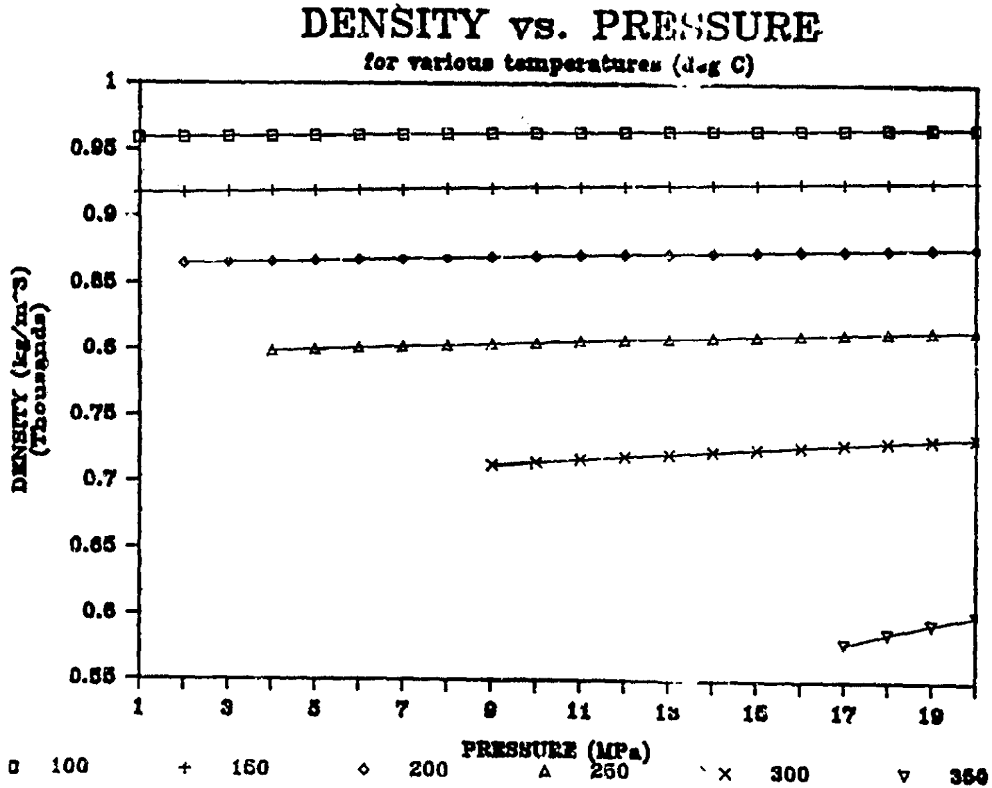
Figure 4.4 Density vs. pressure at various temperatures in subcooled water.
