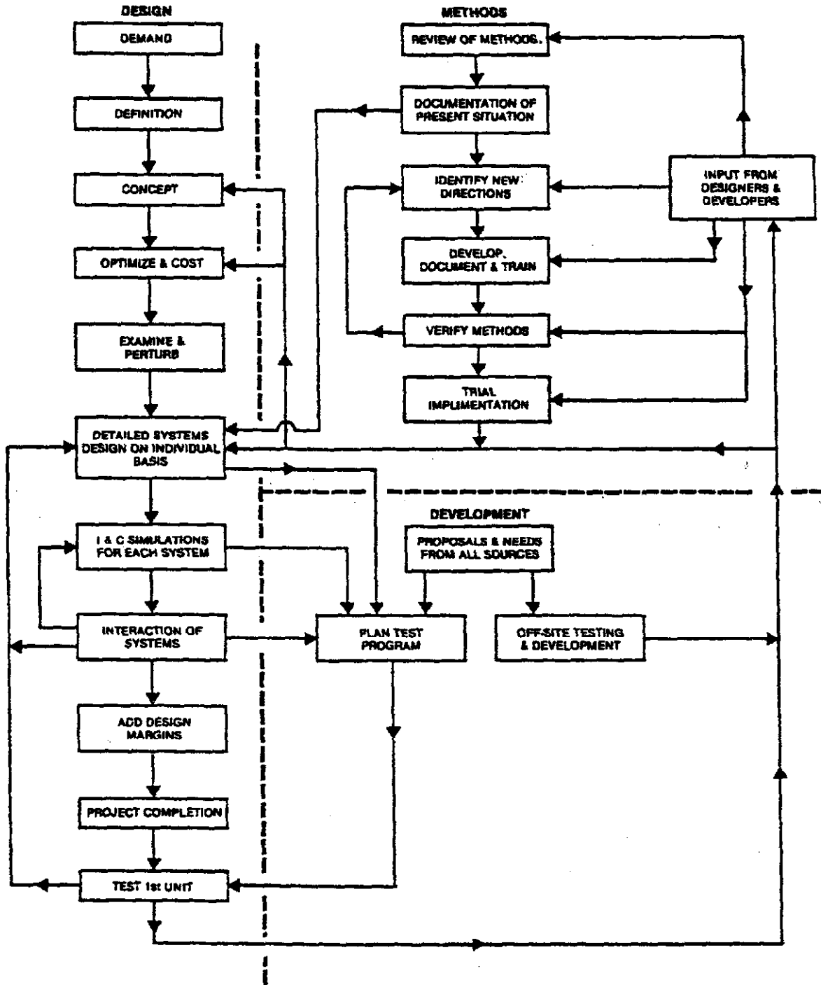
Figure 7.2 Details of the interaction process
