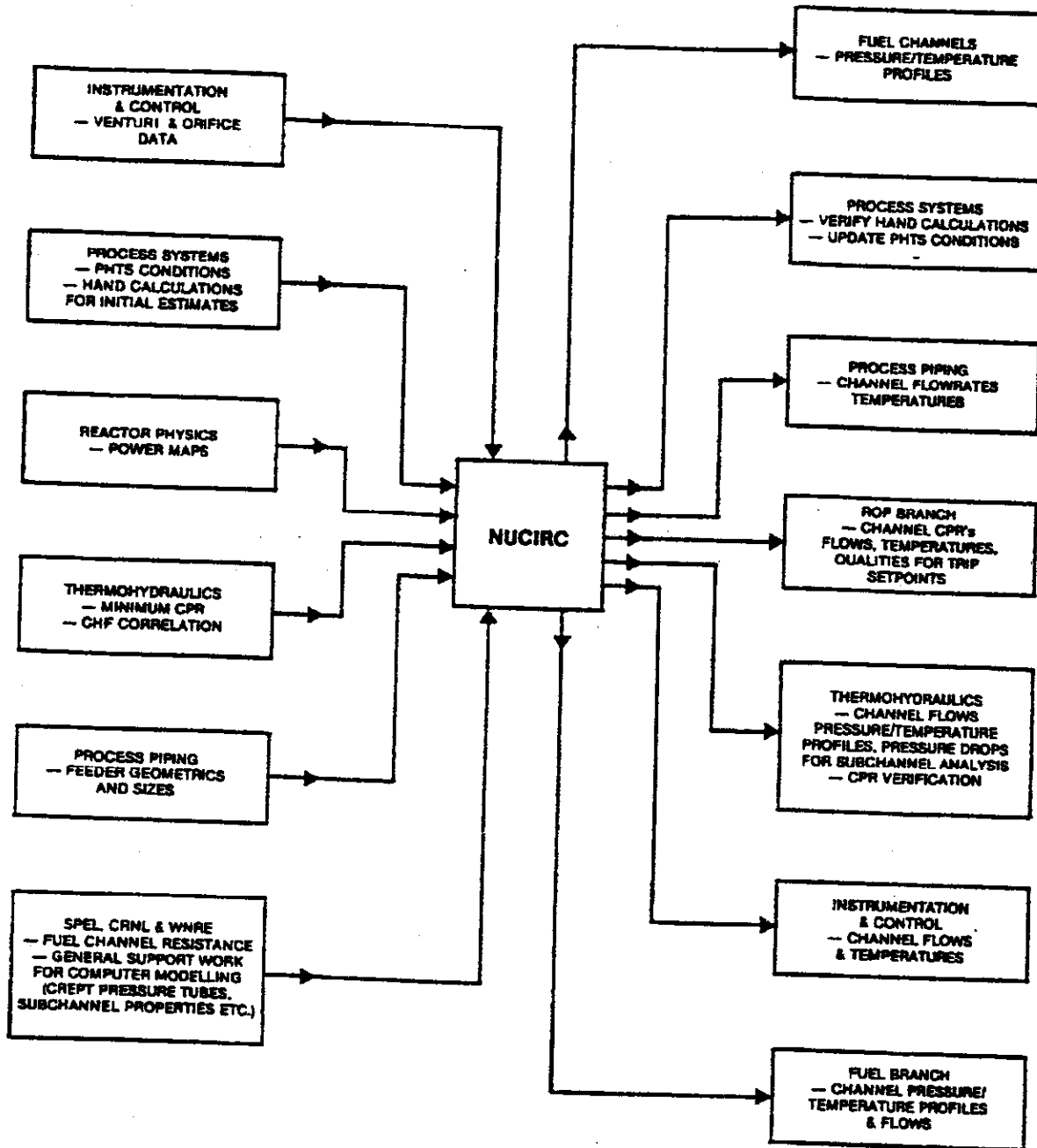
Figure 7.4 NUCIRC interaction
