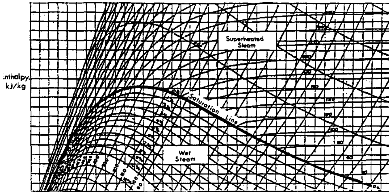
Entropy, kJ/kg °C
