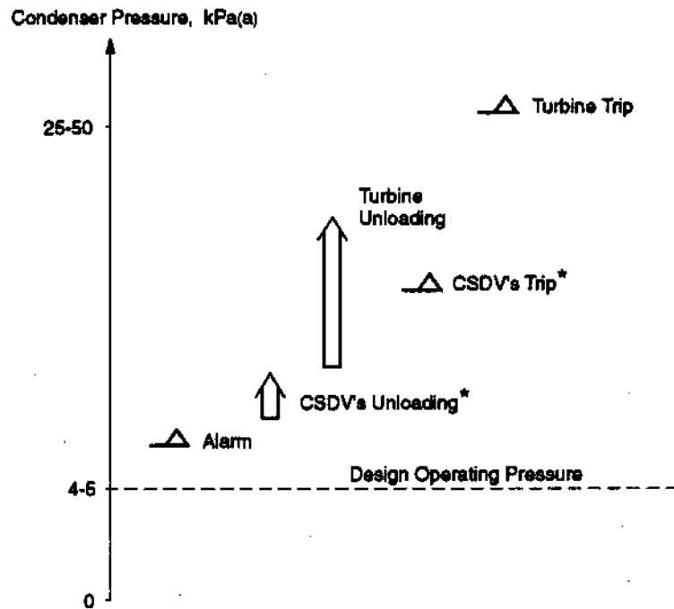
Fig. 5.2. Major automatic responses to high condenser pressure:
