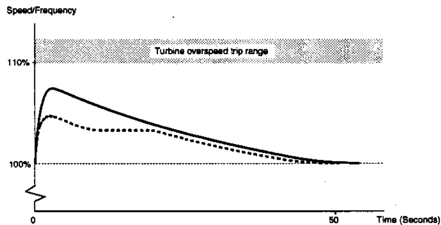
Fig. 3.4. Typical turbine overspeed transient on a full load rejection.
