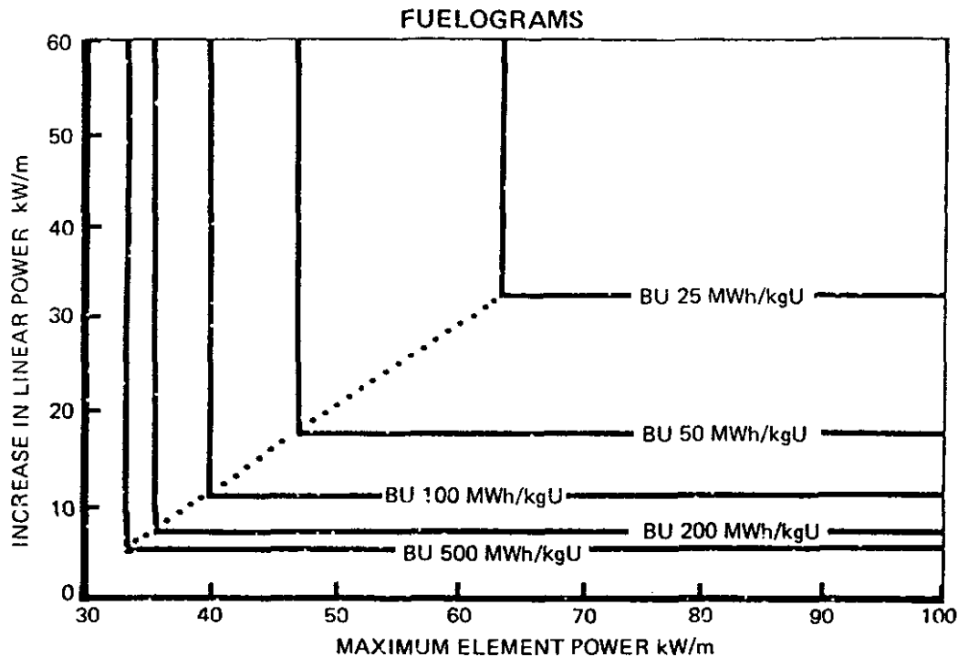
FIGURE 36 Fuelgrams
