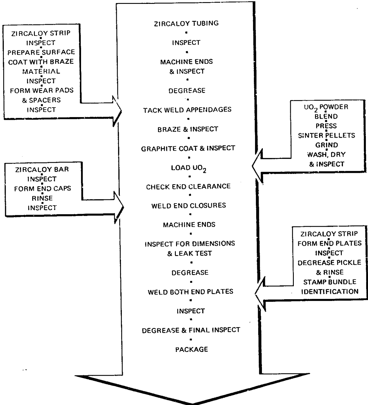
FIGURE 14 Split Spacer Bundle Manufacturing Steps
