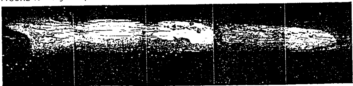
FIGURE 40 High Temperature Corrosion Failure of Fuel Element
