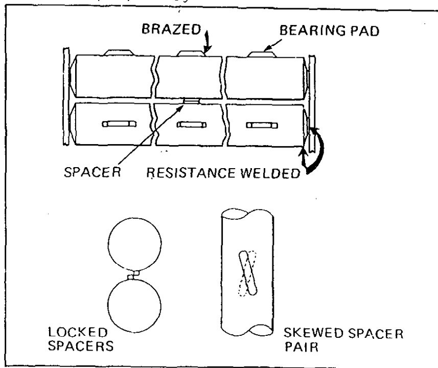
FIGURE 10 Split Spacer Design
