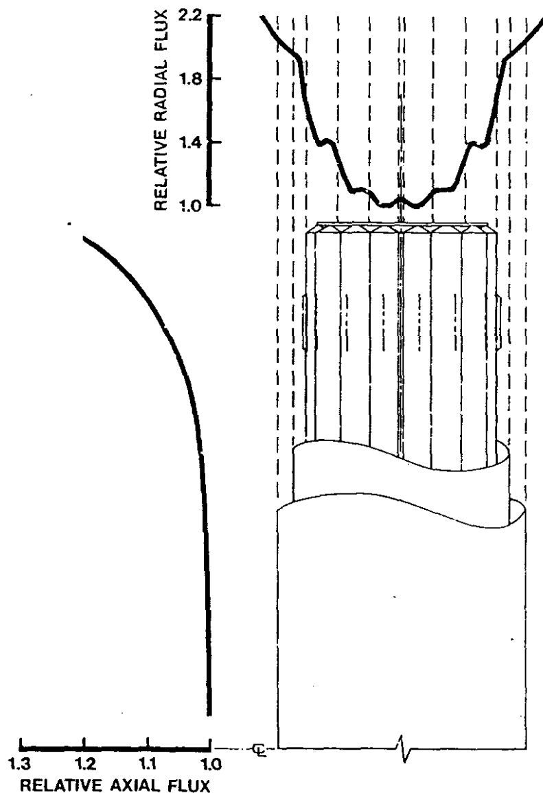
FIGURE 43 Bundle Radial and Axial Flux Distribution
