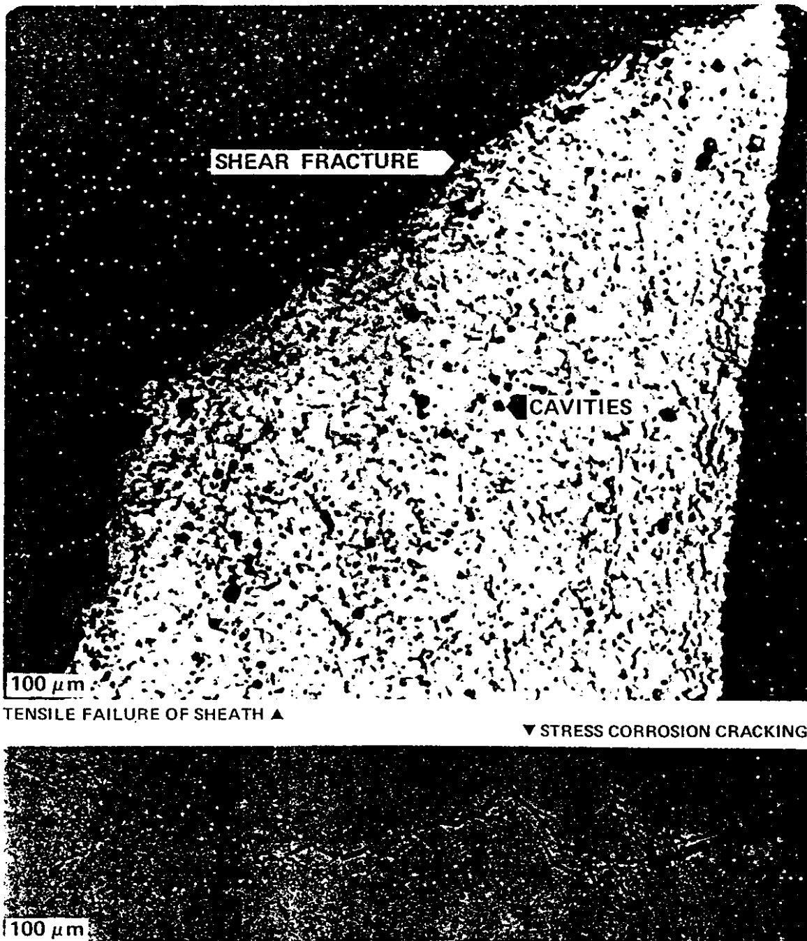
FIGURE 34 Defect Mechanisms
