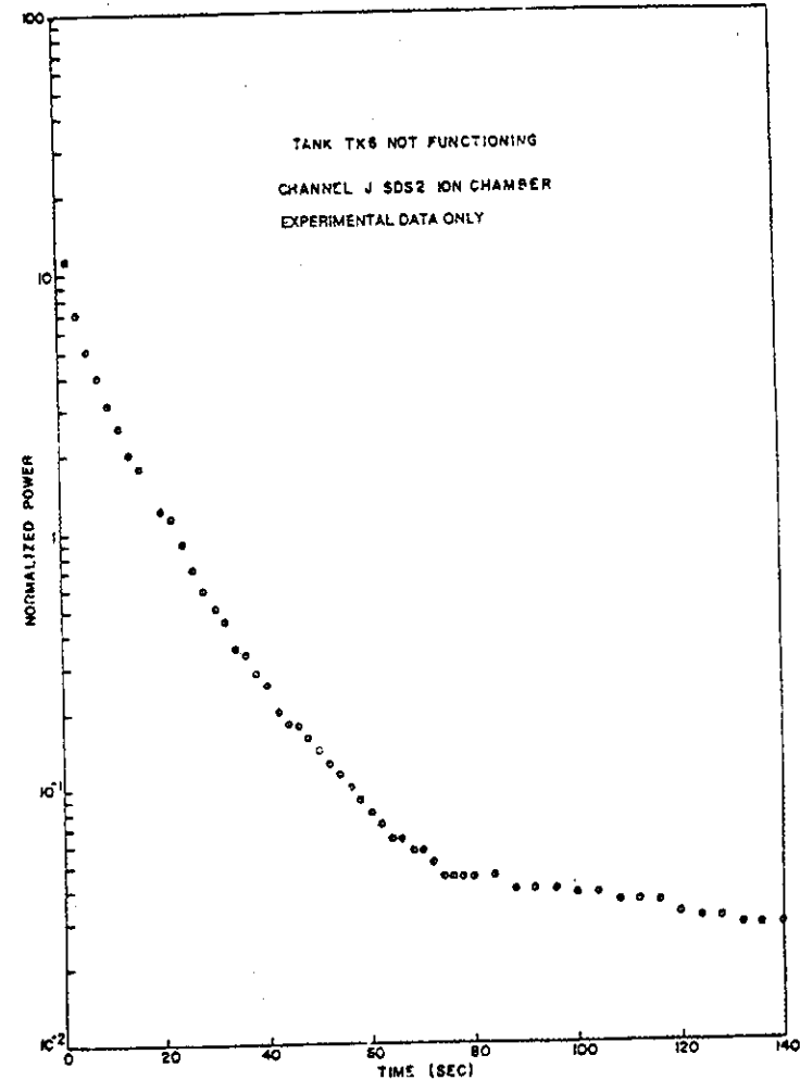
Figure 7-9: SDS#2 Test - 6 Tanks.
