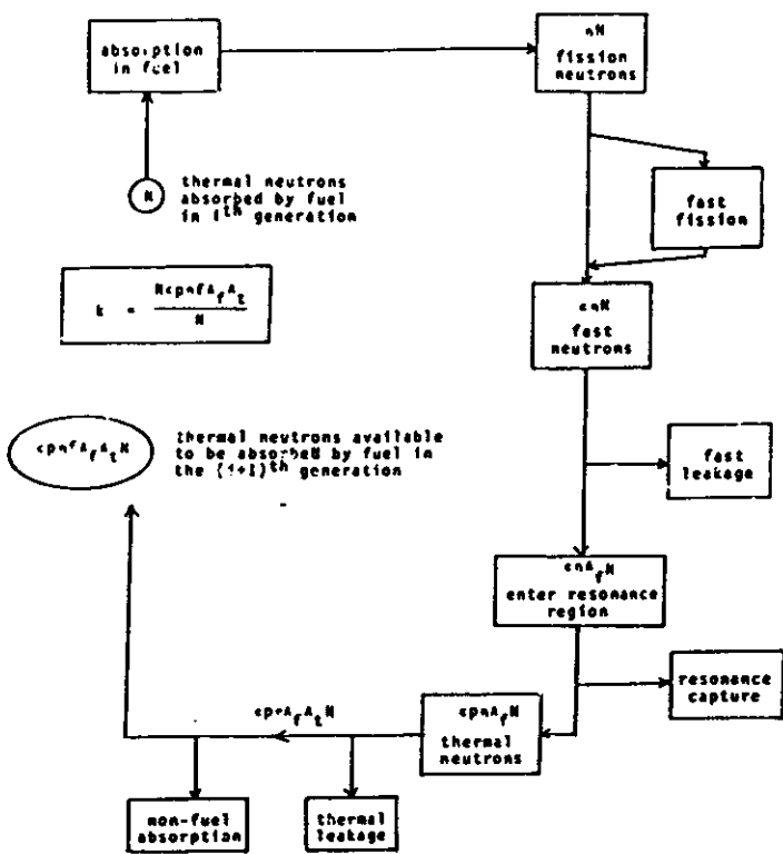
Figure 5.2 Multiplication factor in neutron cycle
