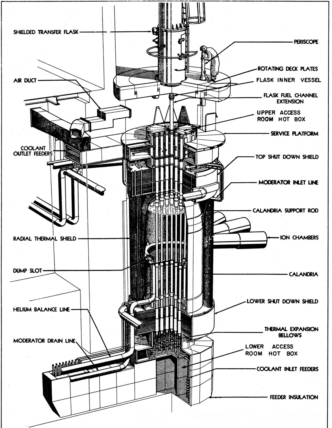
6.2-9 WR-1 REACTOR CUTAWAY
