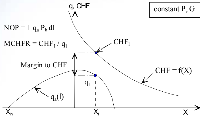
(a) Schematic representation of definition of MCHFR
