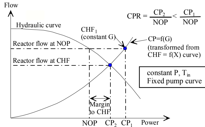
(c) Schematic representation of definition of CPR
