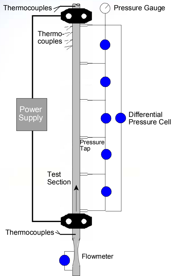
Direct Heating
