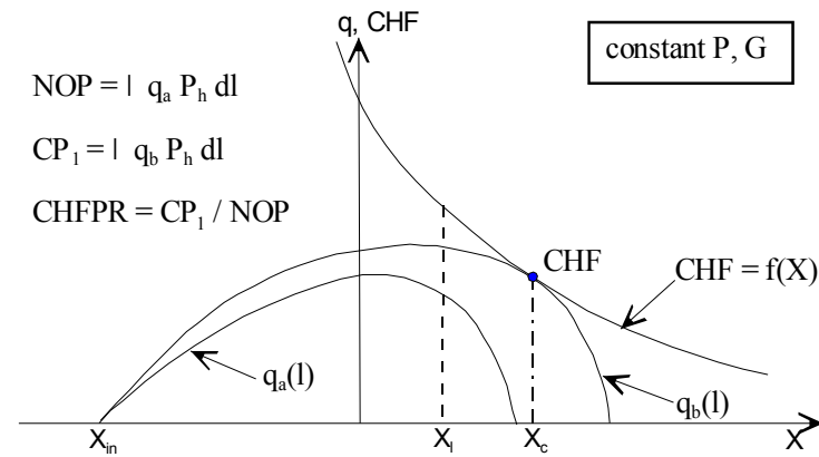
(b) Schematic representation of definition of CHFPR
