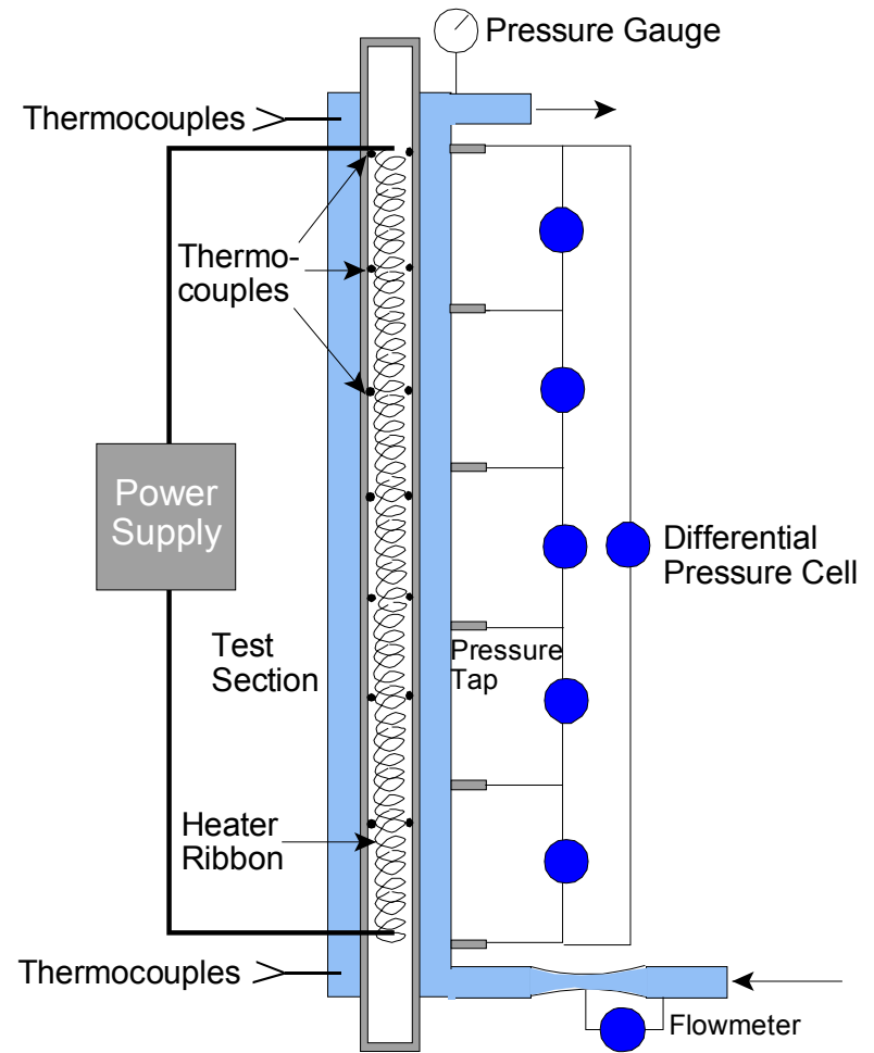
Indirect Heating
